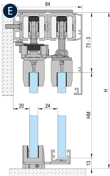
Wandmontage / 2-vleugelig
