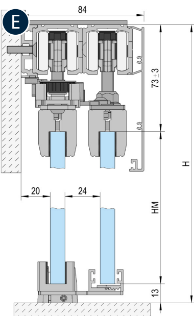
Wandmontage / 2-flüglig
